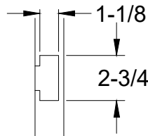
T Strike
