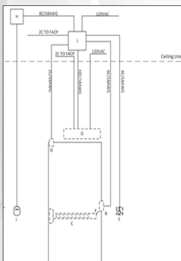
RISER DIAGRAMS
