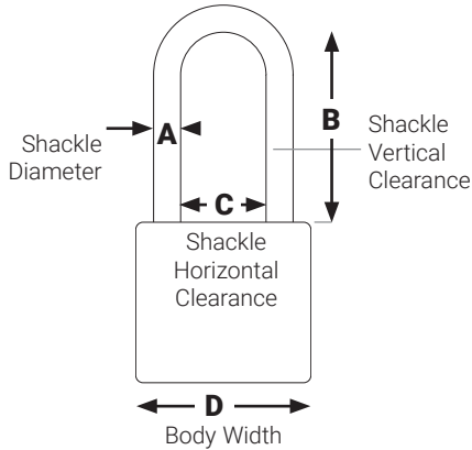
Shackle Dimensions
