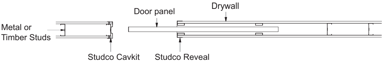
CavKit with Closer Cap (Plan view)
