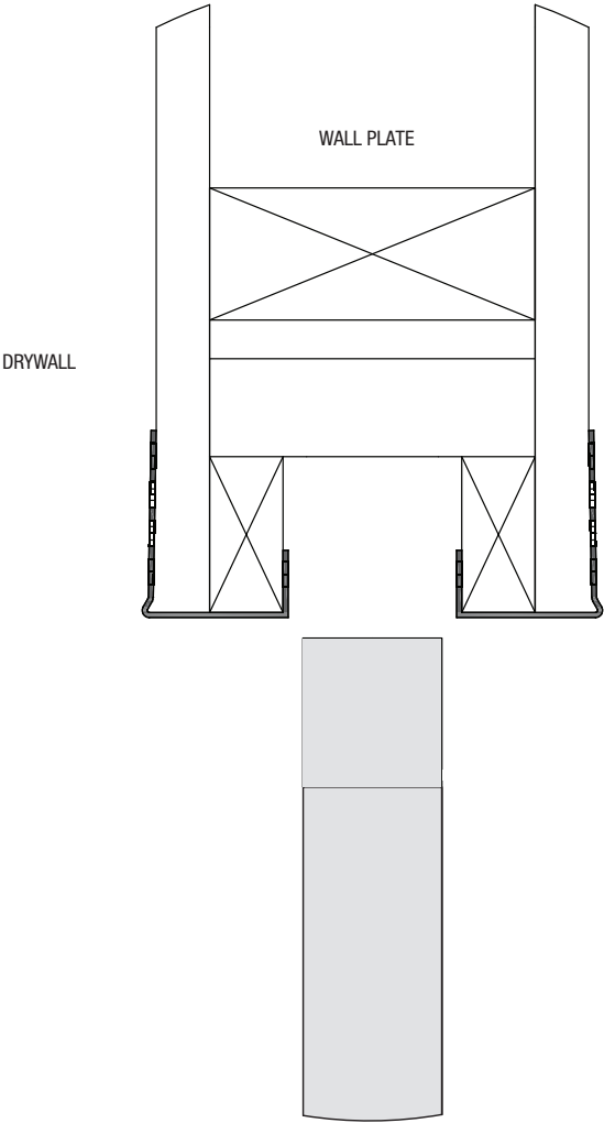
CavKit Head Detail (section)
