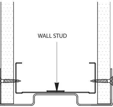
CavKit with Closer Cap (Plan view)
