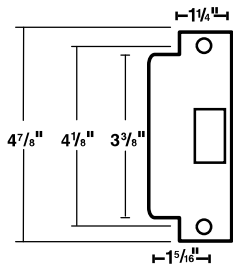
Model No. YR02030* ANSI 4-7/8 Strike with Screw Pack Optional strike available. Plastic strike dust box available separately.
